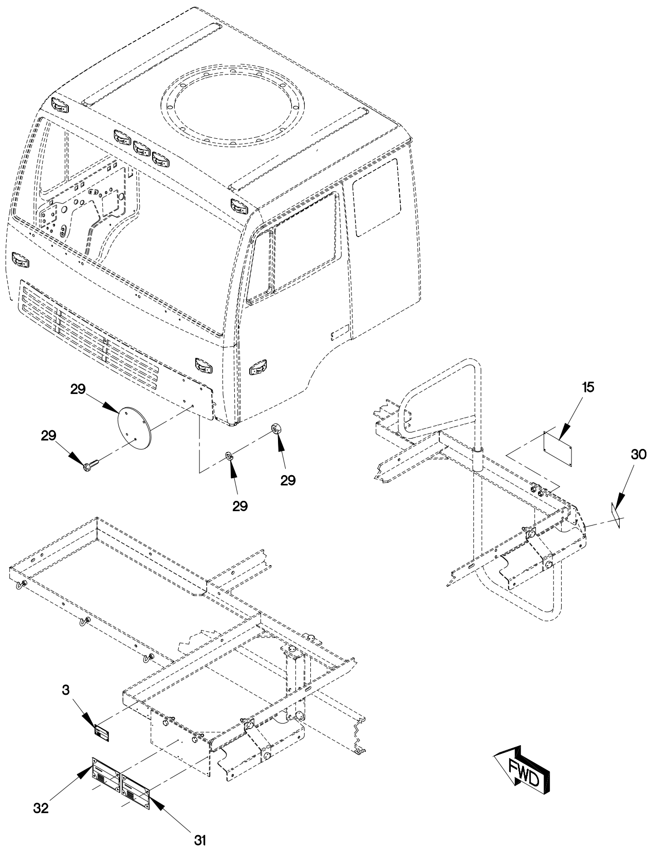
FIGURE 434. DATA AND IDENTIFICATION PLATES (SHEET 6 OF 6)
