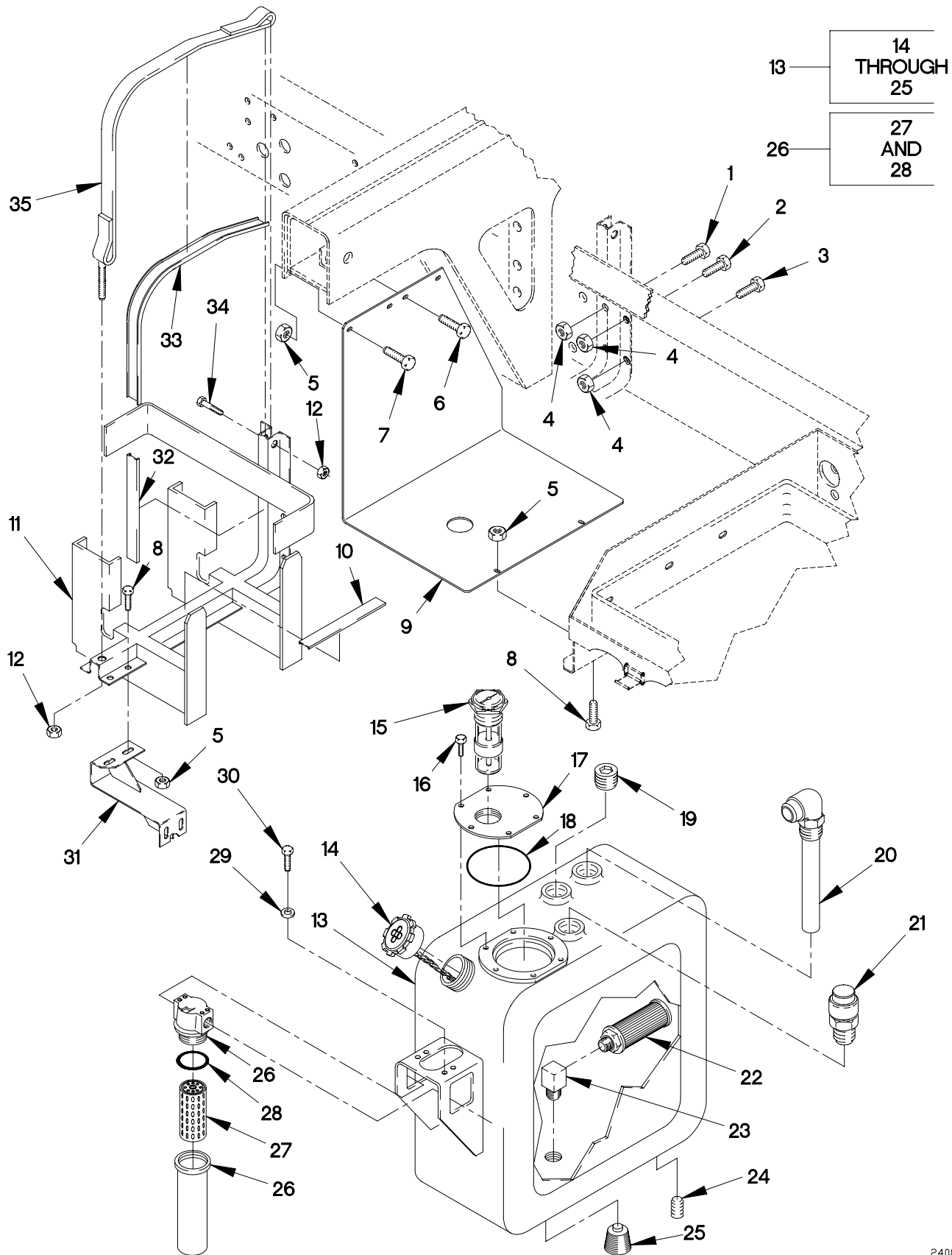
FIGURE 453. HYDRAULIC RESERVOIR AND FILTER
