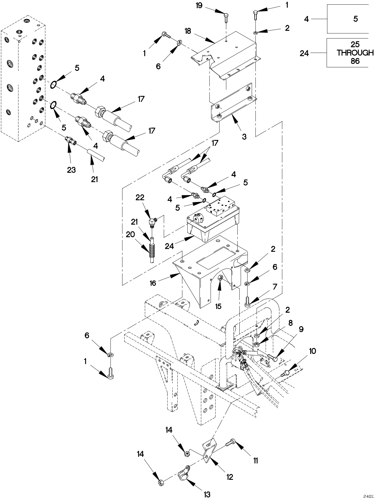
FIGURE 437. AIR/HYDRAULIC POWER UNIT, HOSES AND FITTINGS (SHEET 1 OF 2)
