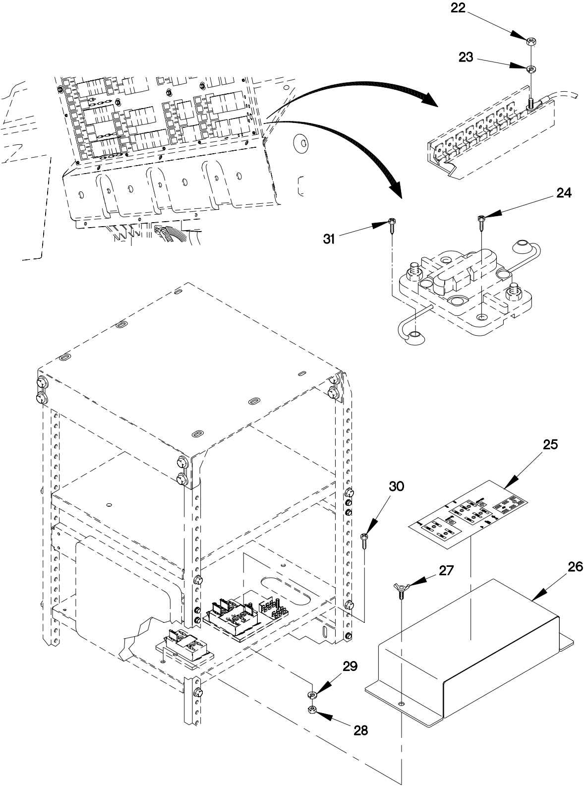
FIGURE 478. DIGITIZATION ELECTRICAL KIT (SHEET 2 OF 2)
